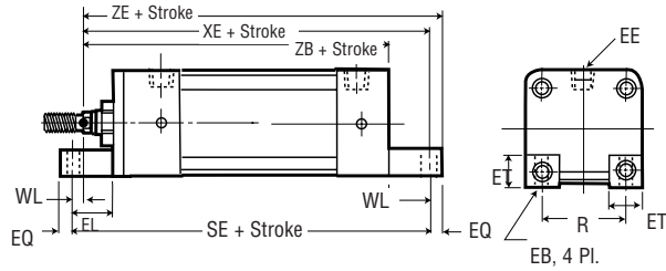
Angle Mount MS1 MOUNT A
