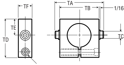
Trunnion
