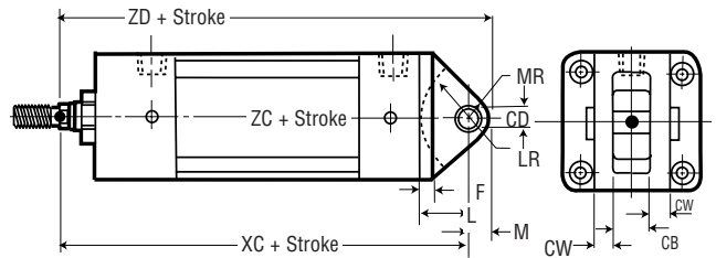
Detachable Eye MP4 MOUNT K
